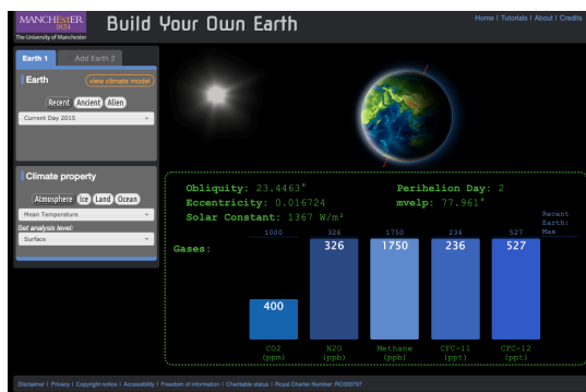
Figure 2: The startup screen for the model. The principle control panels are on the left side of the screen. The central display shows the square meter received by the Earth (solar constant), factors controlling the climate (orbital eccentricity), and principle greenhouse gases that affect the energy balance of the climate, h
