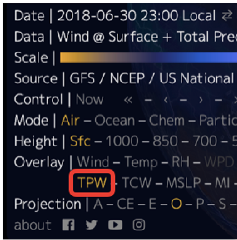
Figure 1 – Display control panel with initial selections highlighted. Figure 2 shows a map of the United States with precipitation data. Areas in blue are wet (high precipitation) while areas in brown are dry (low precipitation).
