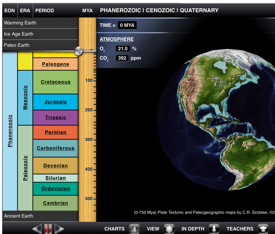
Figure 1 – Default screen for Earth viewer. The multi-colored chart on the left is an interactive time scale / time scale. The task bar across the bottom contains information. Additional controls and data displays appear above the globe.
