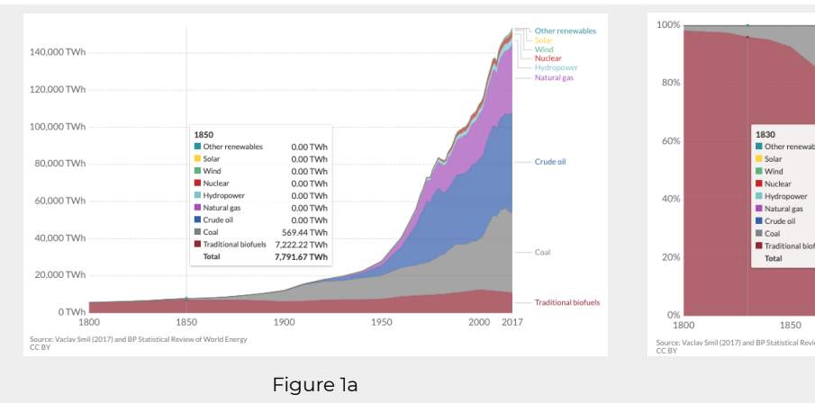
Figure 1 – Global primary energy consumption in Terrawatt-hours between 1800 and 2017 (Figure 1a). You can access the graph in 1b by checking on the “Relative” tab. The graph shown in 1a. In both figures an information panel showing energy consumption for selected years appears when you scroll over the graph.
