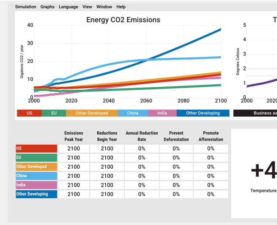
Figure 1 – The default screen for C-ROADS: Most of the controls are located in the upper left corner of the screen. Additional controls include the controls that control the timing and rate of emission reductions, deforestation, and afforestation. The graph on the left shows CO2 emissions per year from 2000 to 2100 and the graph on the right shows the increase in MGT (mean global temperature) for the same time period.
