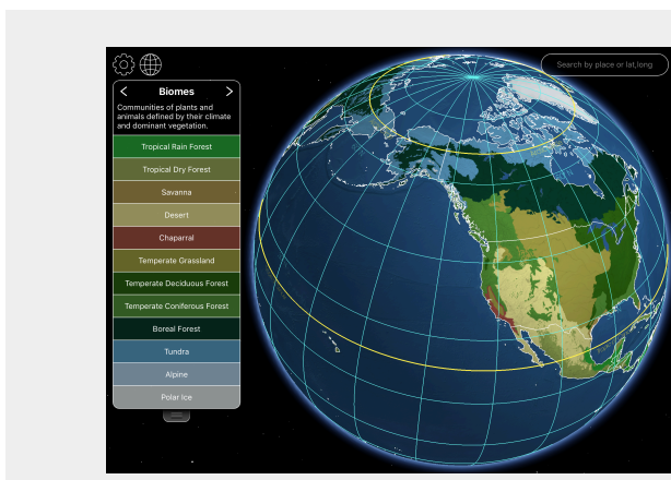
Figure 2 – Default screen for Biome Viewer. The panel to side of the globe lists the major biomes of the planet. Click on any of the labels for a brief description of that biome.
